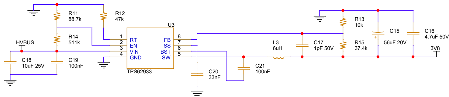
6-18V UNREG BUS TO ADDITIONAL RAIL (VOUT CAN BE ADJUSTED VIA THE FB VOLTAGE DIVIDER)
